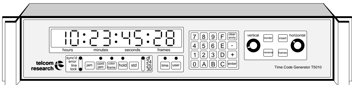
Figure 3.1: T5010 Front Panel
