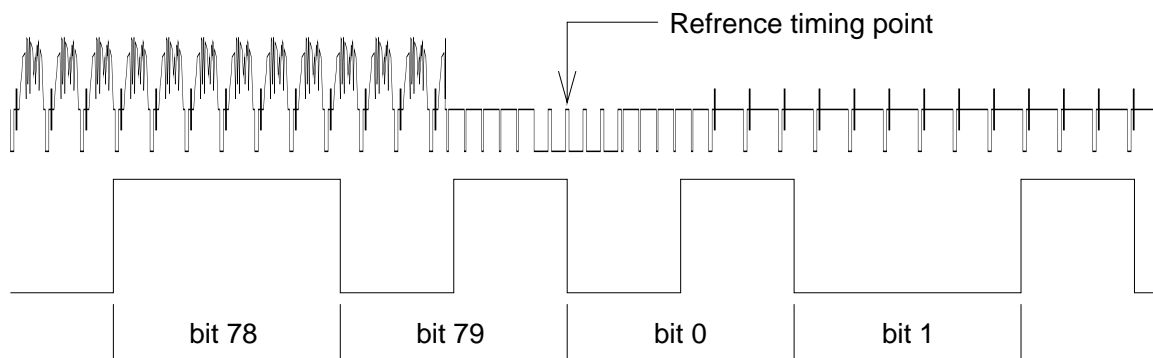
Figure 1.3: Timing Relationship Between EBU Video and Time Code
