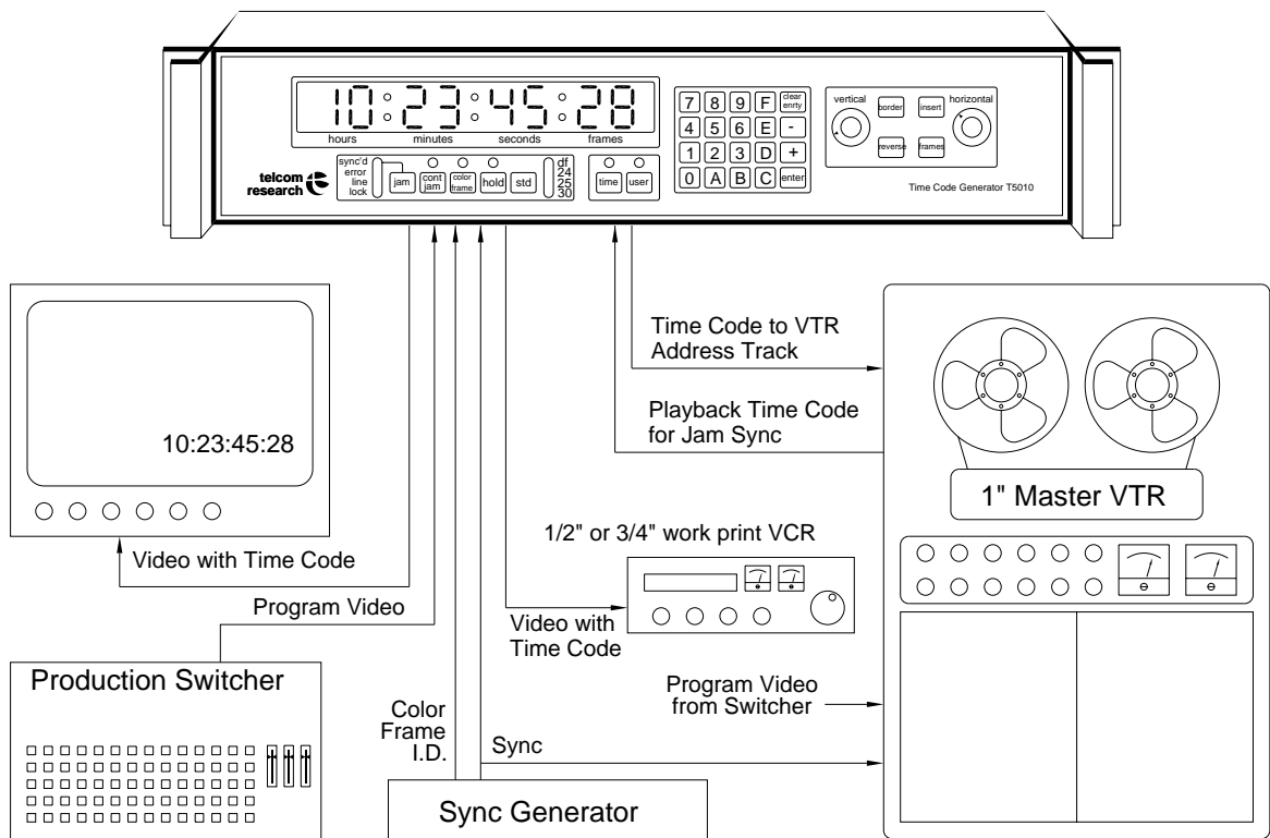
Figure 4.1: Typical Installation of the T5010
