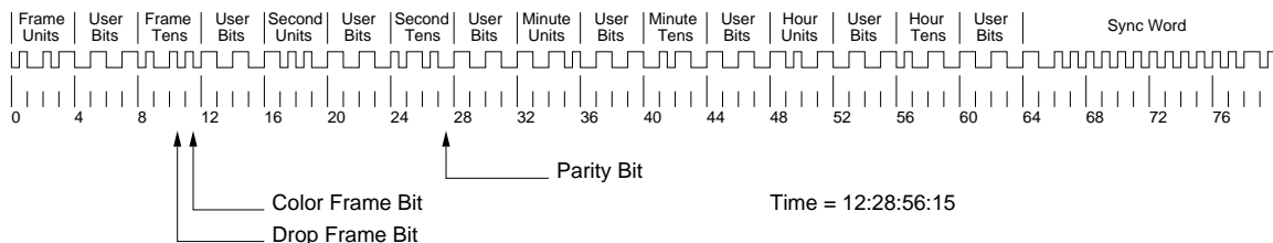
Figure 1.4: Longitudinal Time Code Waveform
