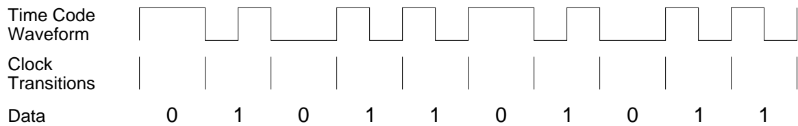
Figure 1.1: Bi-Phase Mark encoding
