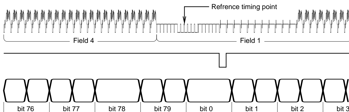
Figure 1.7: Relationship Between Video, Color Frame Identification Pulse and Time Code
