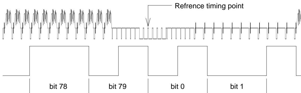
Figure 1.2: Timing Relationship Between NTSC Video and Time Code
