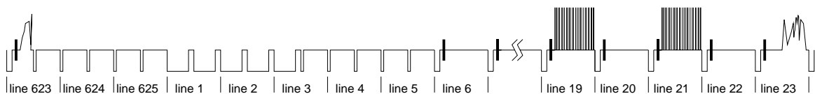
Figure 1.6: EBU Vertical Interval Time Code Waveform
