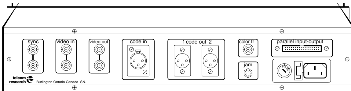
Figure 2.1: T5010 Back Panel
