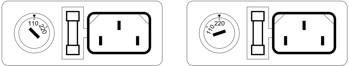
Figure 2.2: T5010 Line Voltage Selector
